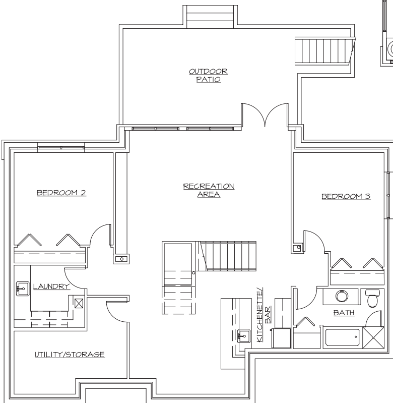
LOWER LEVEL PLAN v
