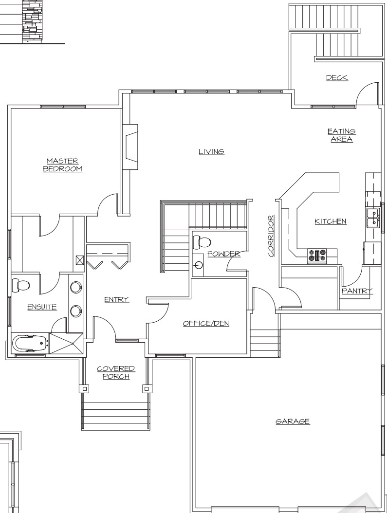
MAIN FLOOR PLAN > 1602 SQ FT
