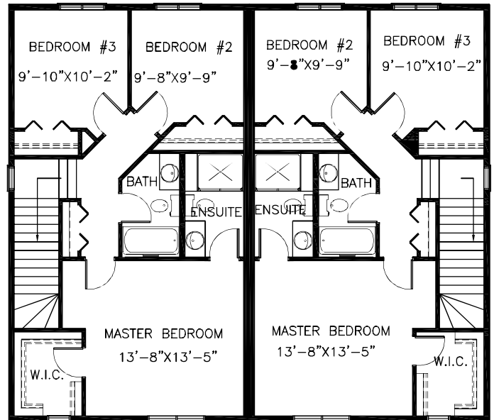
SECOND LEVEL PLAN 748.5 SQ FT (PER UNIT)
