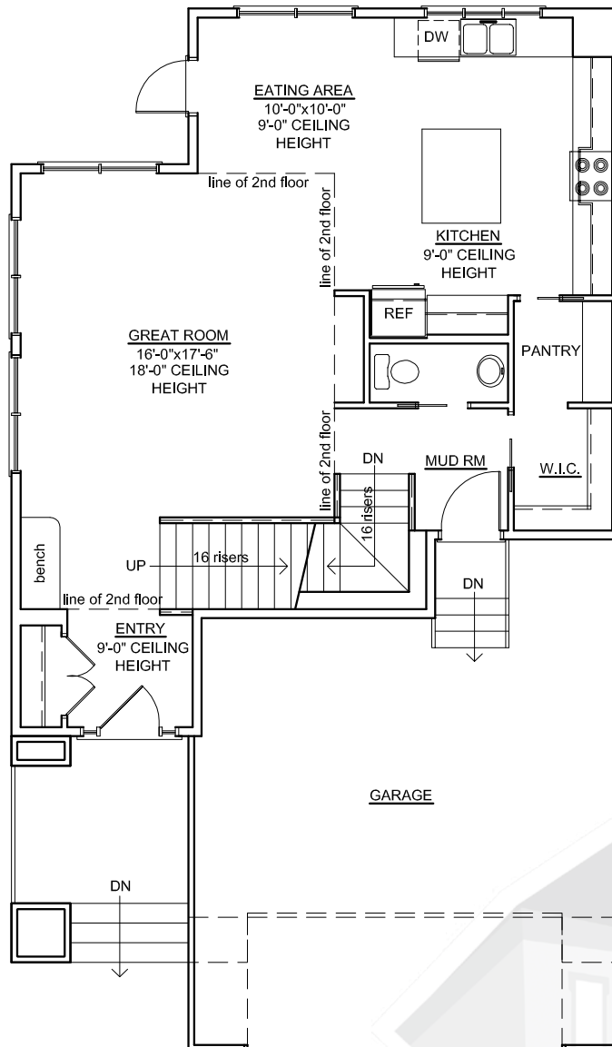
MAIN FLOOR PLAN 1805 SQ FT < OVER FOR SECOND FLOOR
